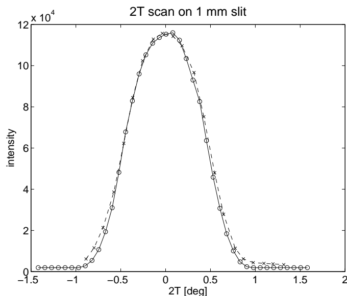
Figure 8.4: Scans of 2\theta_s in the direct beam with 1 mm slit on the sample position. "x": measurements, "o": simulations Collimations: open-30'-open-open.
